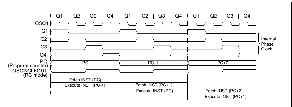
FIGURE 3-5: CLOCK/INSTRUCTION CYCLE
