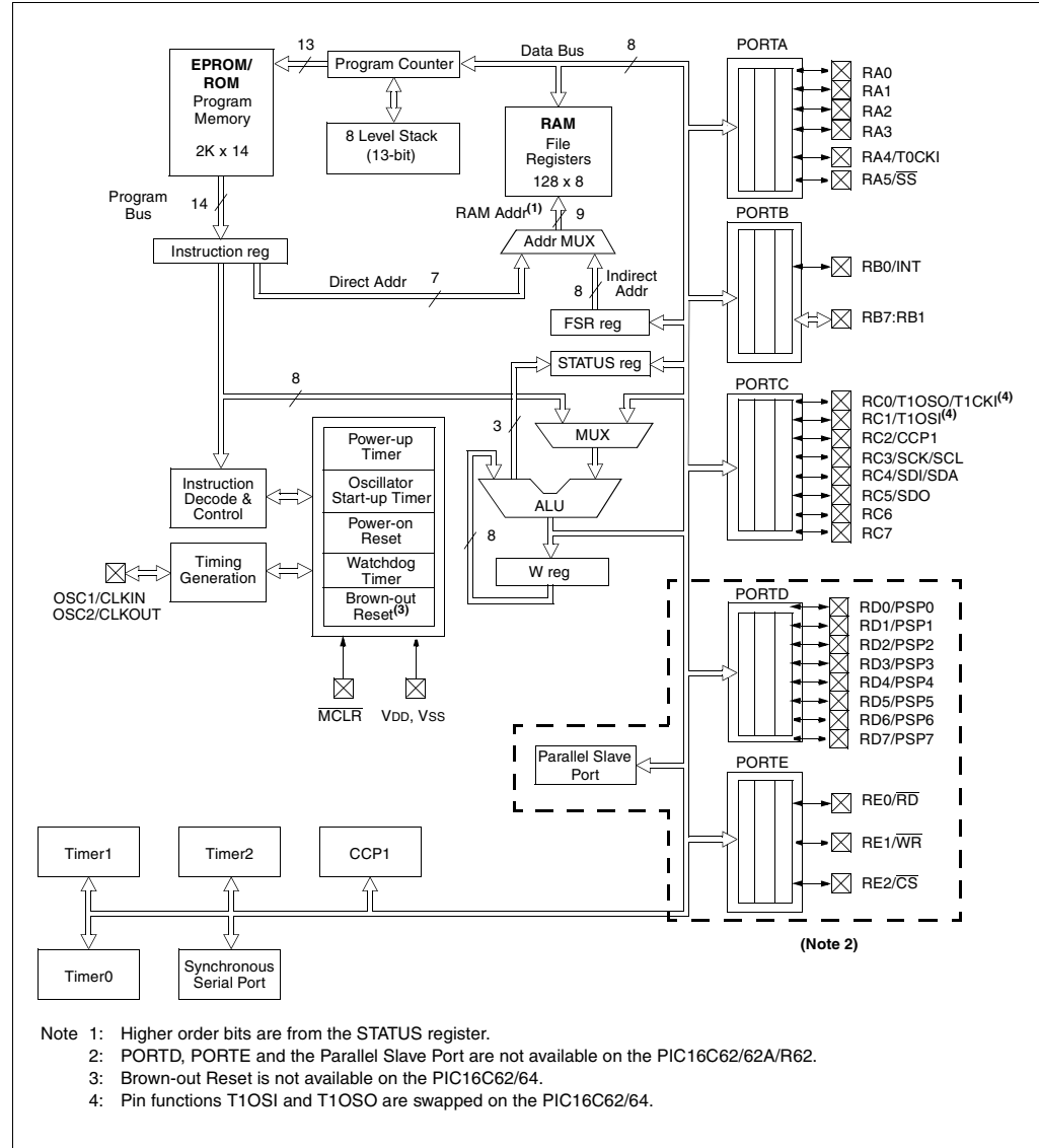
FIGURE 3-2: PIC16C62/62A/R62/64/64A/R64 BLOCK DIAGRAM
