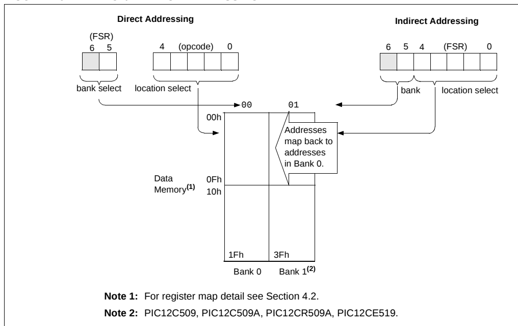
FIGURE 4-9: DIRECT/INDIRECT ADDRESSING
