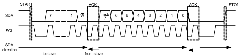
Figure 23 - Write transaction
