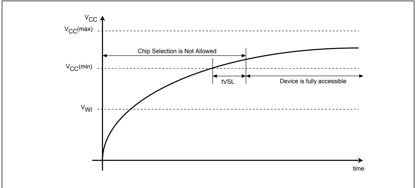
Figure 67. Power-up Timing
