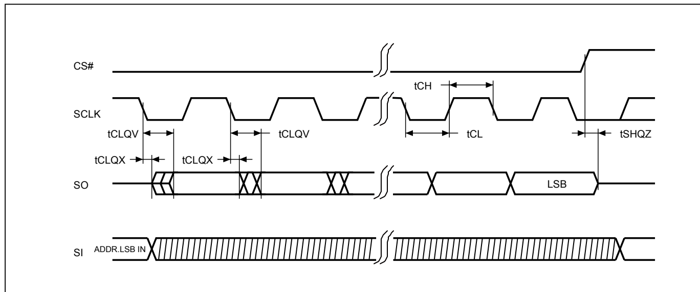
Figure 10. Output Timing
