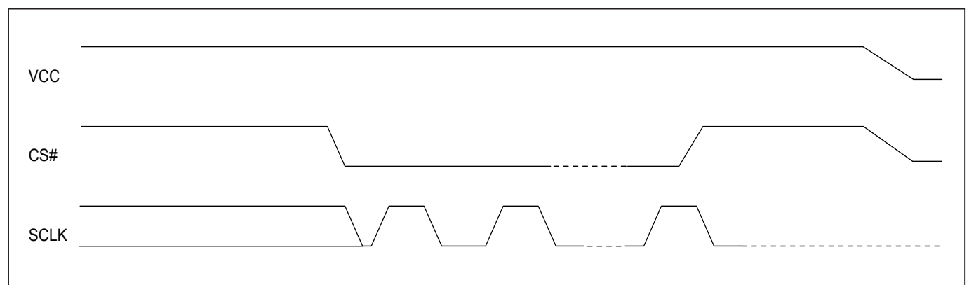
Figure 28. Power-Down Sequence
