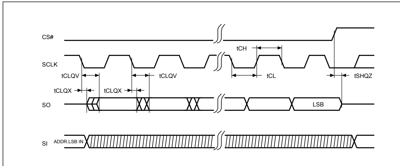
Figure 10. Output Timing
