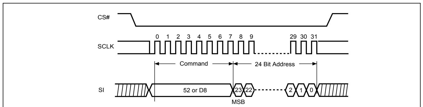
Figure 21. Block Erase (BE) Sequence (Command 52h or D8h)
