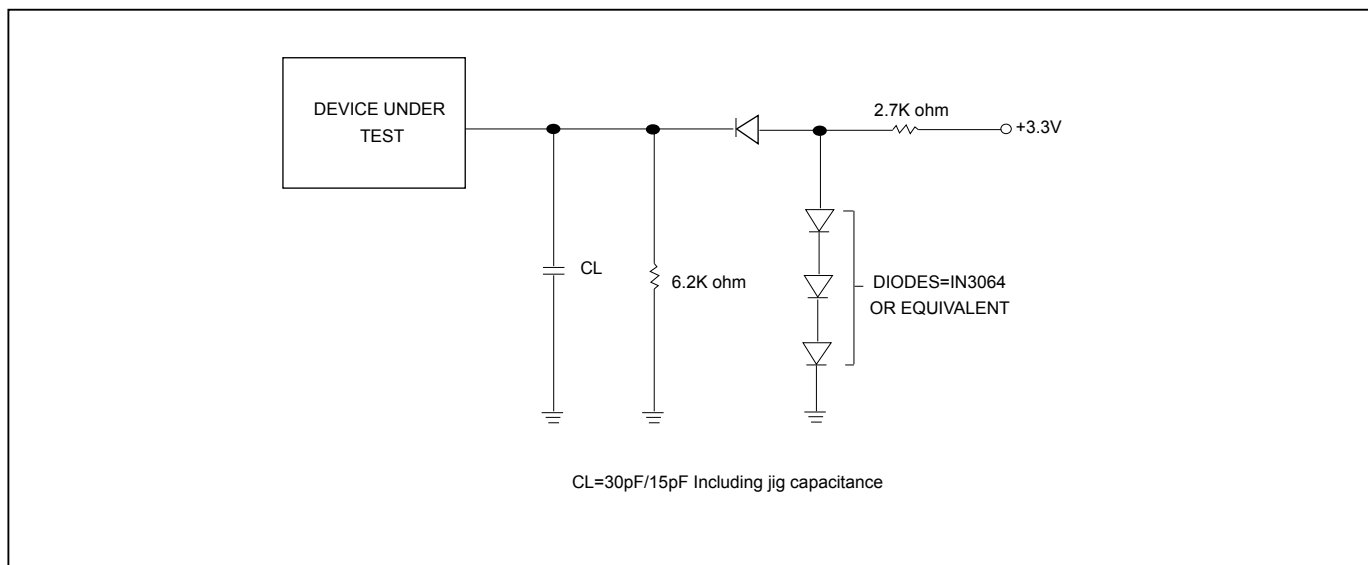
Figure 7. OUTPUT LOADING
