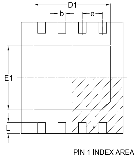
BOTTOM VIEW
