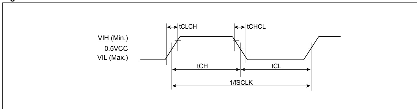
Figure 8. SCLK TIMING DEFINITION
