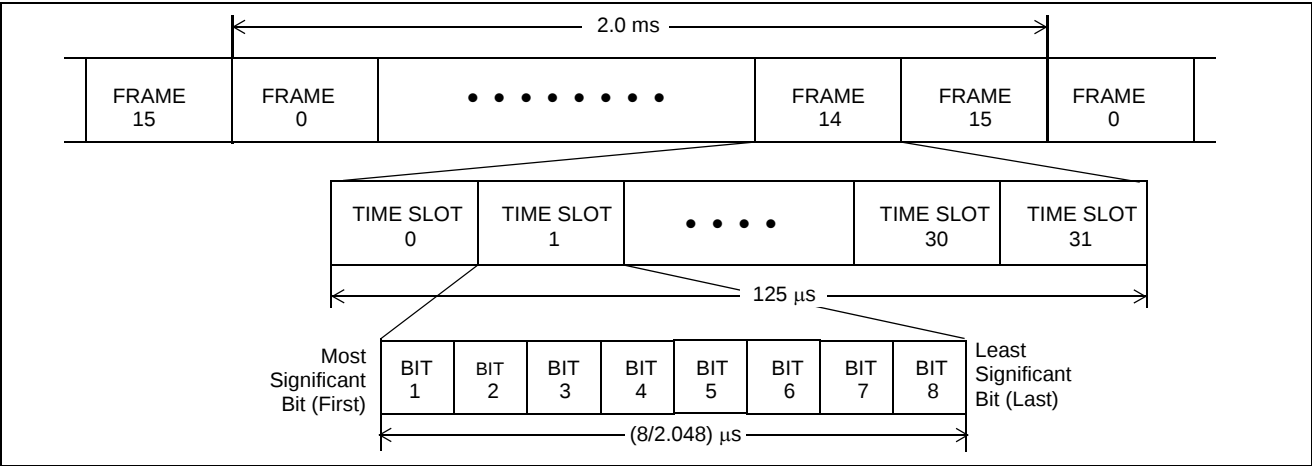
Figure 30 - PCM 30 Format
