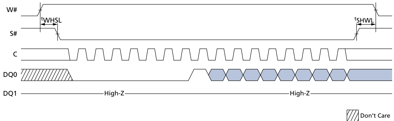
Figure 45: Write Protect Setup and Hold During WRITE STATUS REGISTER Operation (SRWD = 1)
