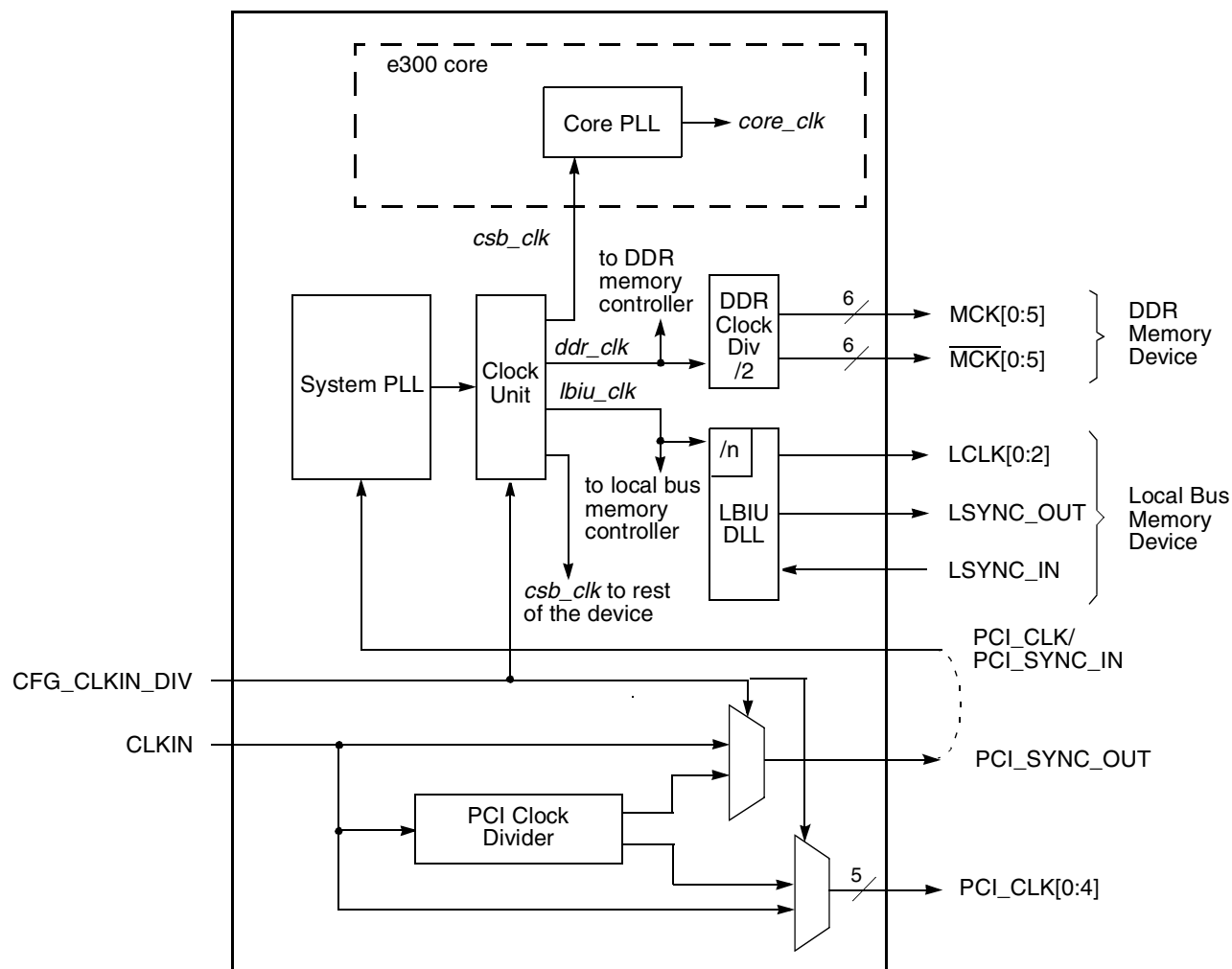
Figure 67. Clock Subsystem
