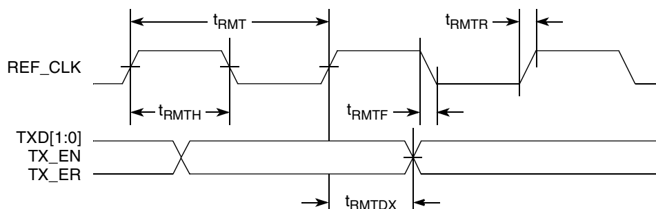
Figure 16. RMI Transmit AC Timing Diagram
