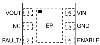
6-Pin 1.6mm x 1.6mm TMLF (MT) (Top View) MIC2095-1YMT/MIC2098-1YMT
