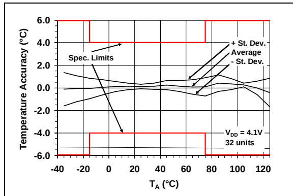
FIGURE 2-1: Temperature Accuracy.
