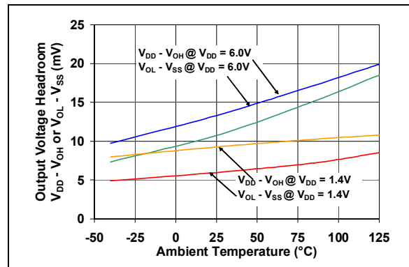
FIGURE 2-23: Output Voltage Headroom vs. Ambient Temperature.
