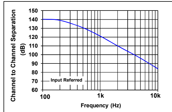
FIGURE 2-32: Channel-to-Channel Separation vs. Frequency (MCP6442/4 only).
