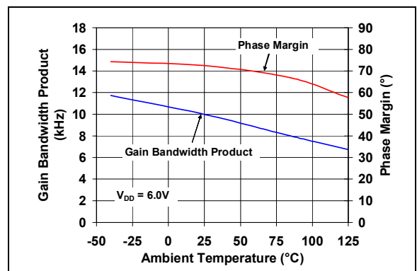
FIGURE 2-18: Gain Bandwidth Product, Phase Margin vs. Ambient Temperature.
