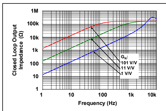
FIGURE 2-30: Closed Loop Output Impedance vs. Frequency.
