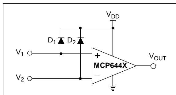
FIGURE 4-2: Protecting the Analog Inputs.
