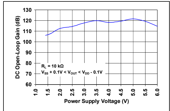
FIGURE 2-16: DC Open-Loop Gain vs. Power Supply Voltage.
