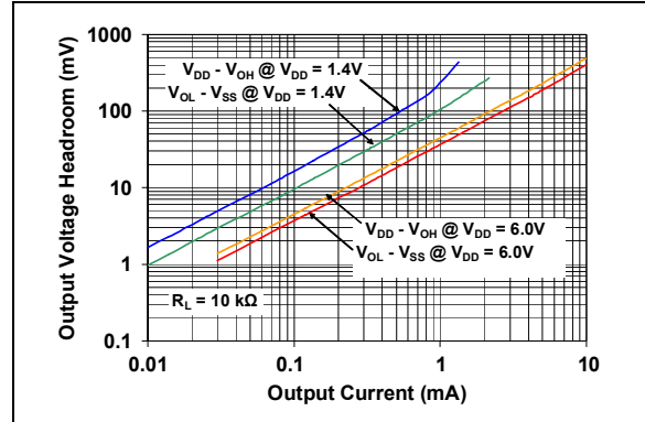
FIGURE 2-22: Output Voltage Headroom vs. Output Current.
