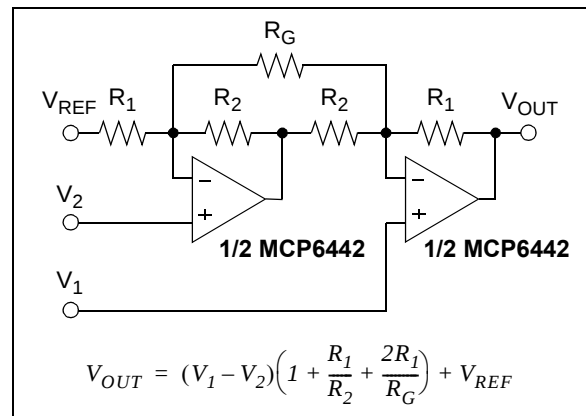
FIGURE 4-9: Two Op Amp Instrumentation Amplifier.
