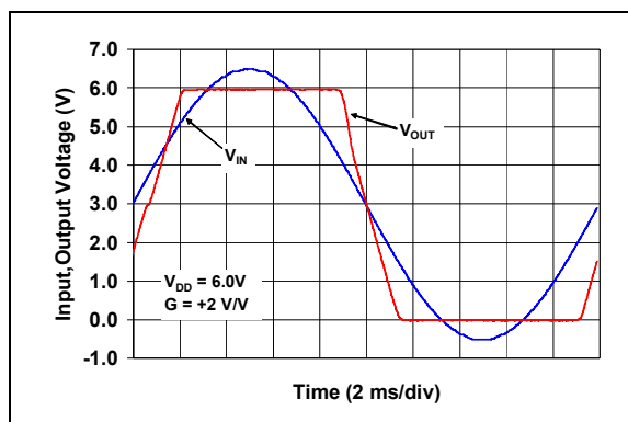
FIGURE 2-29: The MCP6441/2/4 Device Shows No Phase Reversal.
