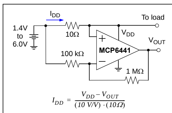
FIGURE 4-7: Battery Current Sensing.
