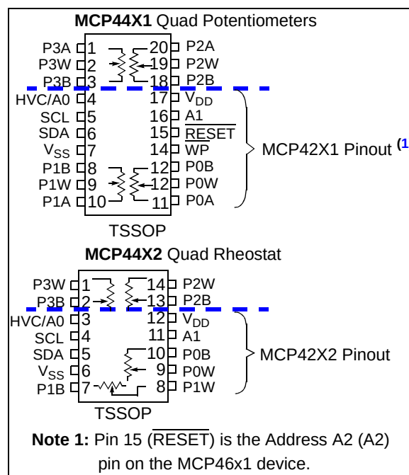
FIGURE 8-7: Quad Pinout (TSSOP Package) vs. Dual Pinout.
