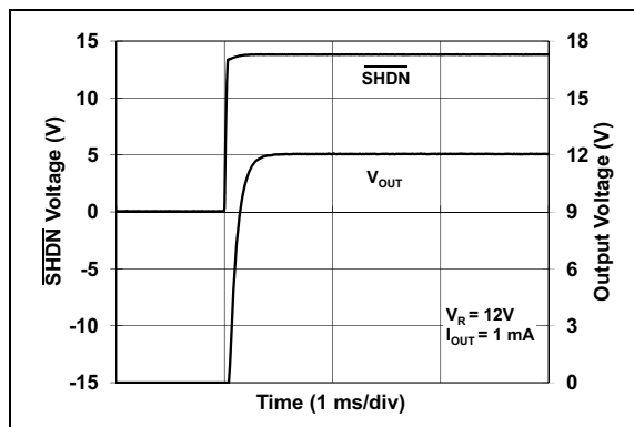
FIGURE 2-42: SHDN Response.
