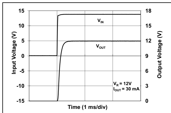
FIGURE 2-39: Start-up Response.
