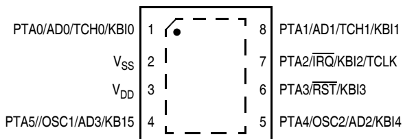
8-PIN ASSIGNMENT MC68HC908QT2 AND MC68HC908QT4 DFN
