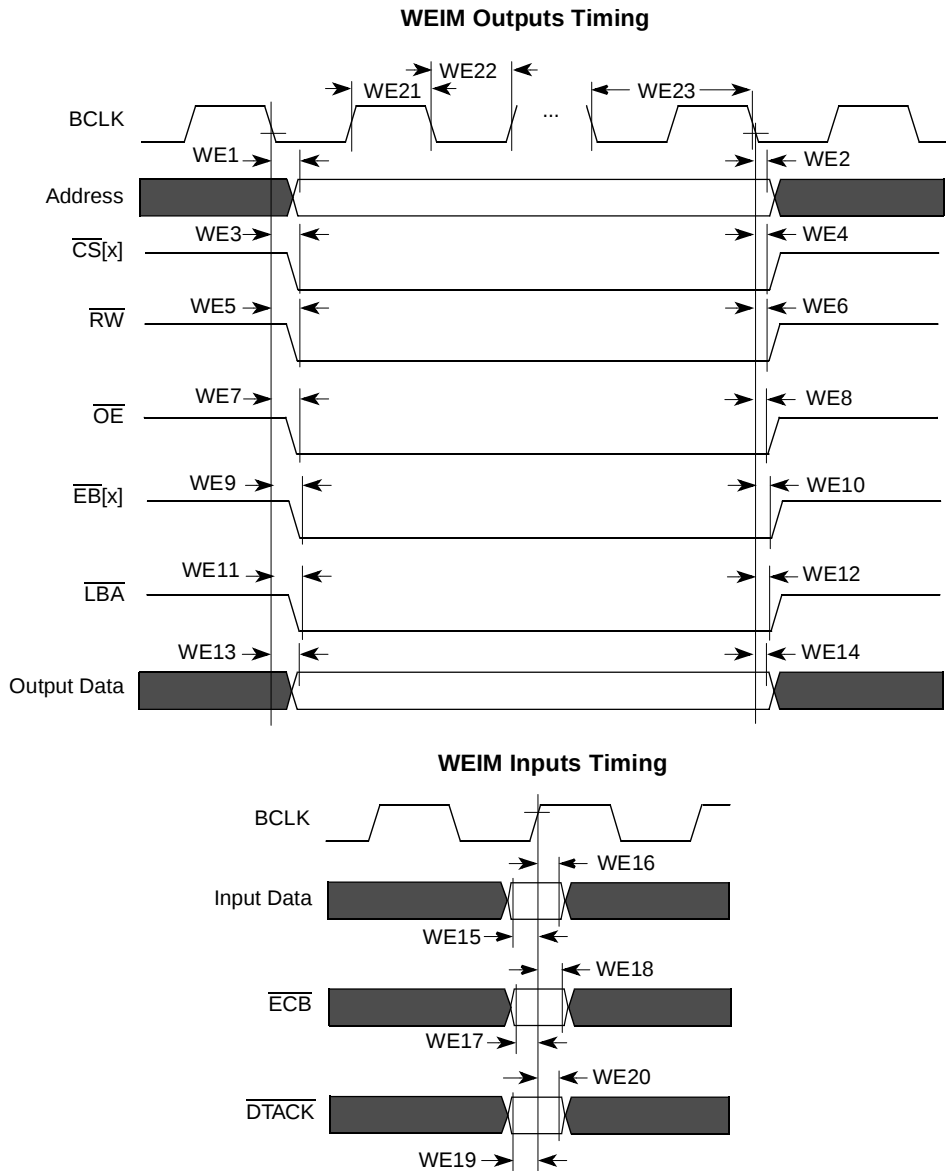
Figure 26. WEIM Bus Timing Diagram
