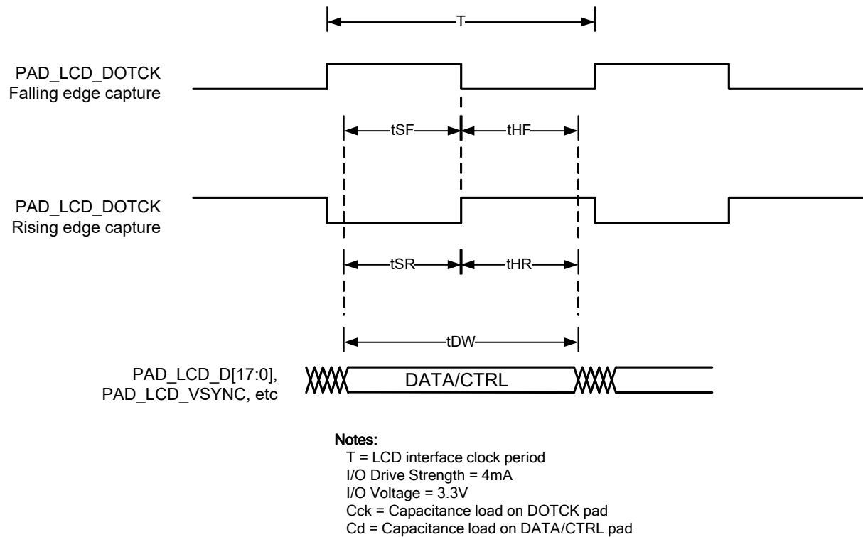
Figure 24. LCD AC Output Timing Diagram
