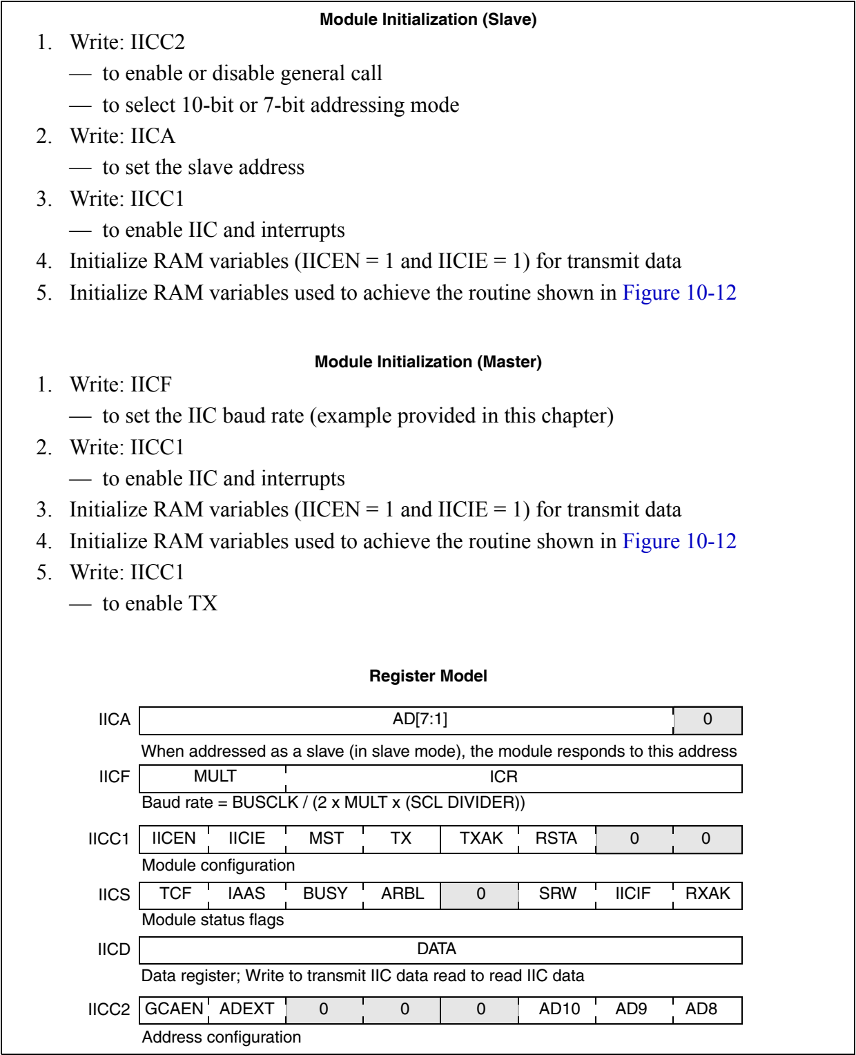
Figure 10-11. IIC Module Quick Start
