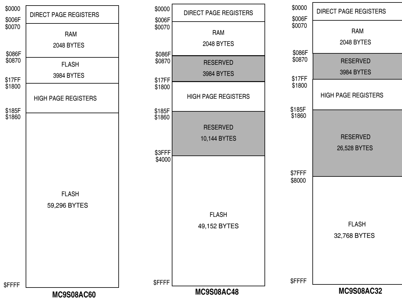
Figure 4-1. MC9S08AC60 Series Memory Map
