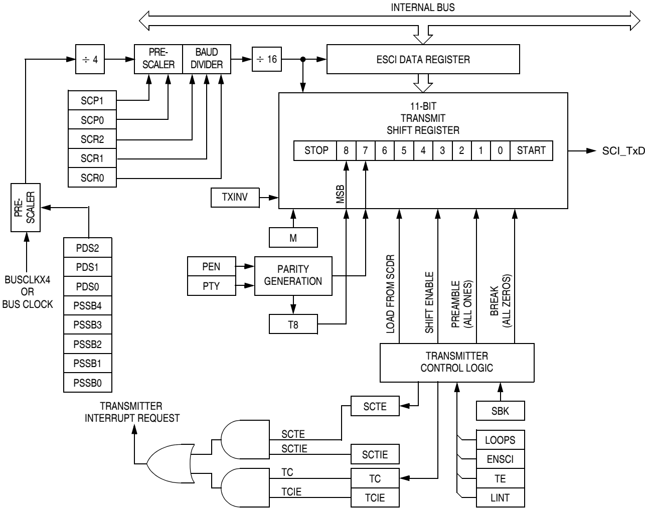
Figure 13-4. ESCI Transmitter
