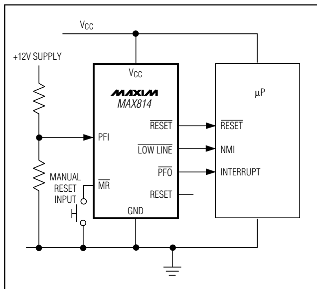
Figure 1b. MAX814 Typical Application
