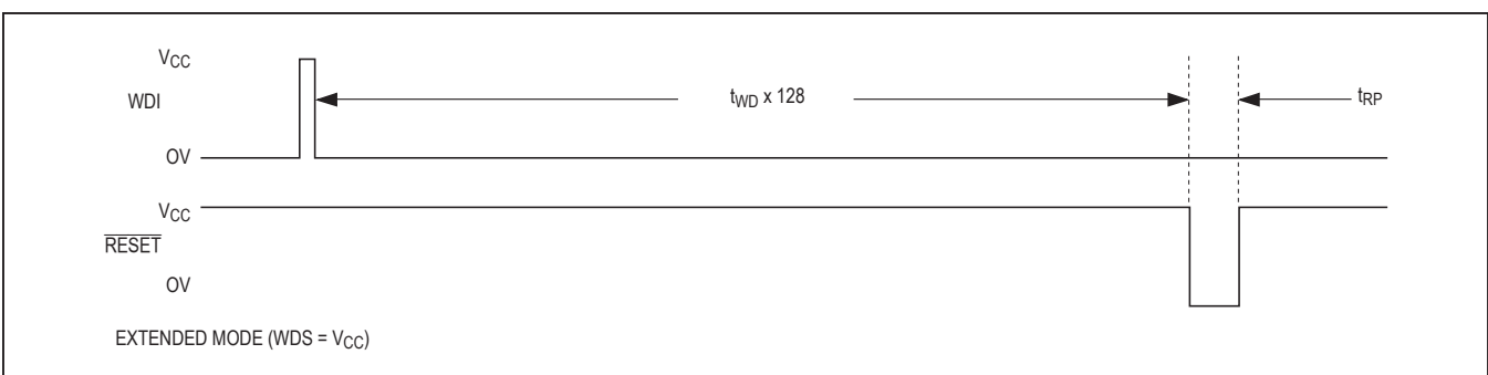
Figure 4b. Watchdog Timing Diagram, WDS = V_{CC}
