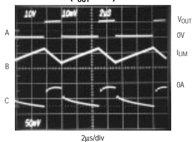
HEAVY-LOAD SWITCHING WAVEFORMS (V OUT = 12V)
