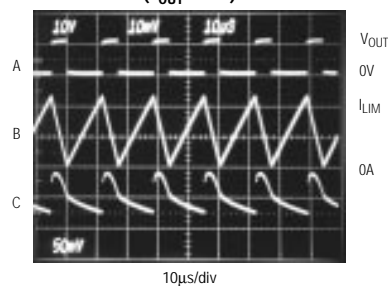
MEDIUM-LOAD SWITCHING WAVEFORMS (V OUT = 12V)
