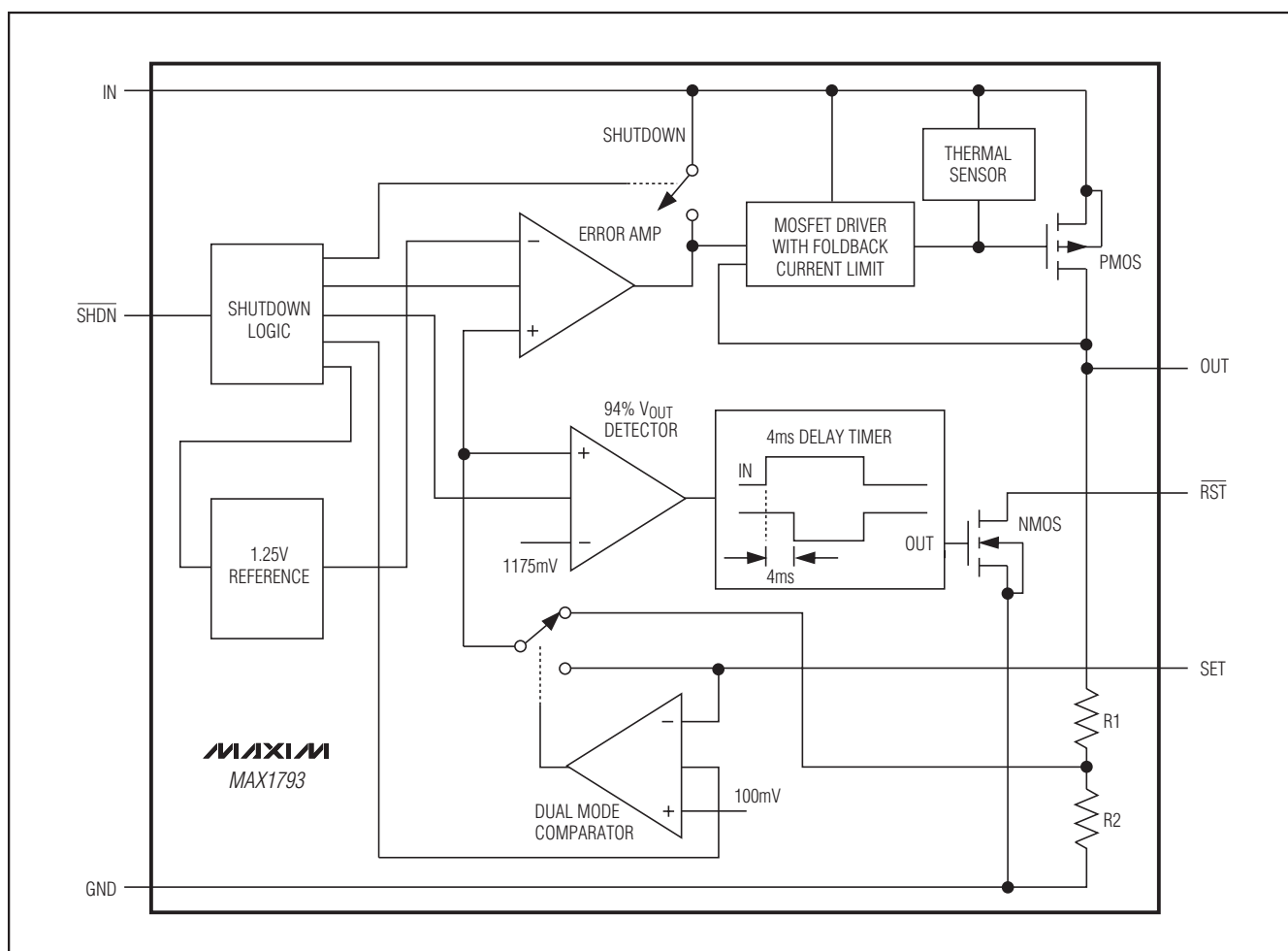
Figure 1. Functional Diagram
