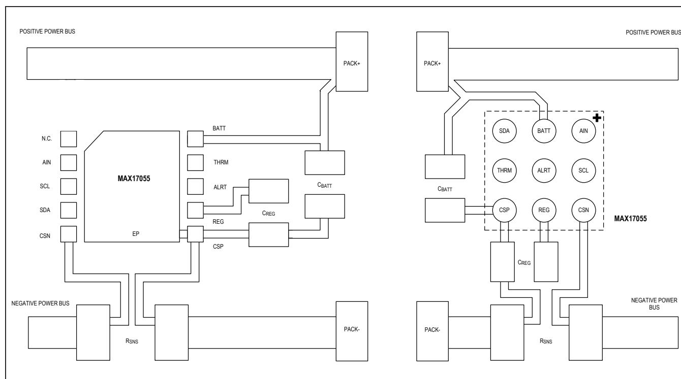
Figure 4. Layout Examples
