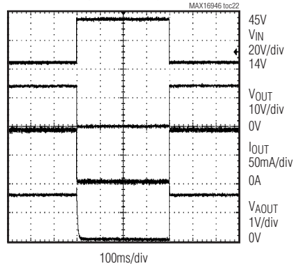
HIGH-VOLTAGE LINE TRANSIENT RESPONSE (MAX16947)
