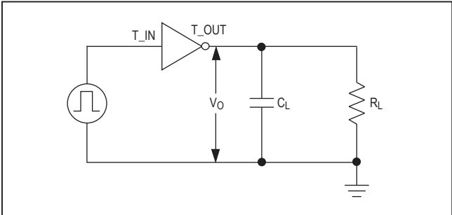
Figure 1. Driver Test Circuit
