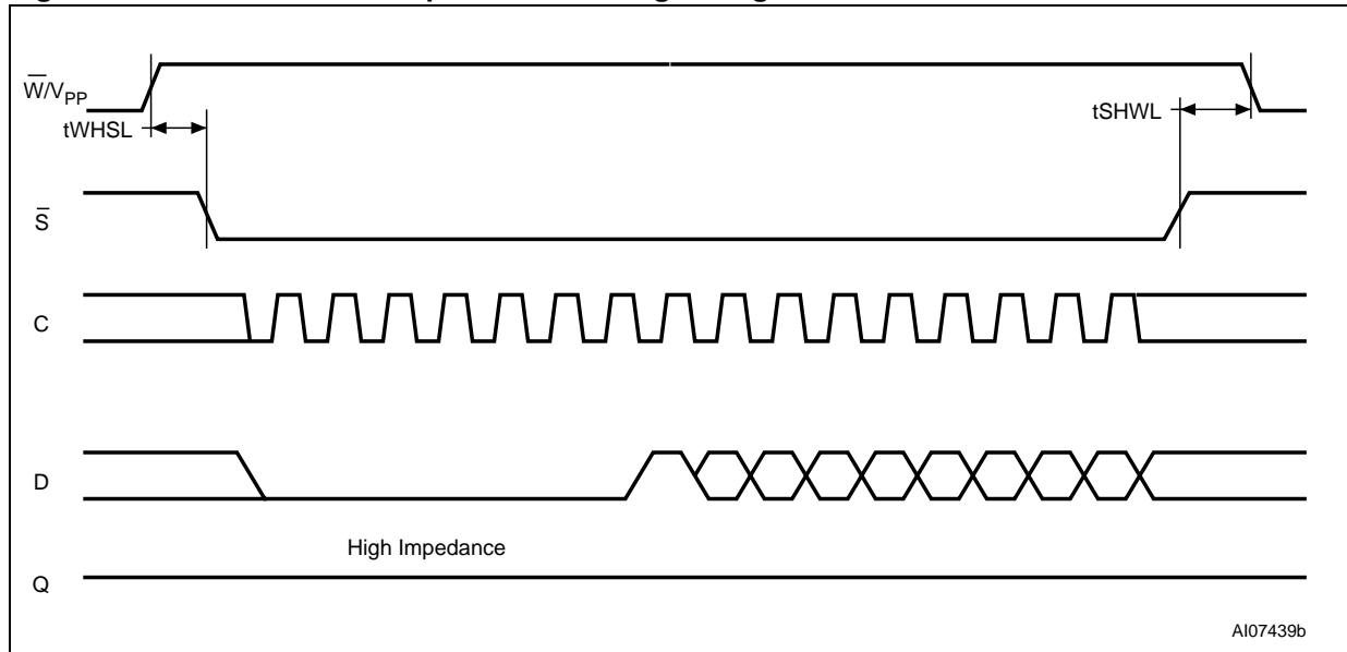
Figure 24. Write Protect Setup and Hold timing during WRSR when SRWD=1
