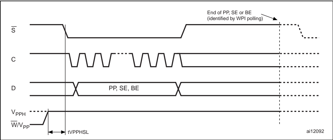
Figure 27. V_{PPH} timing
