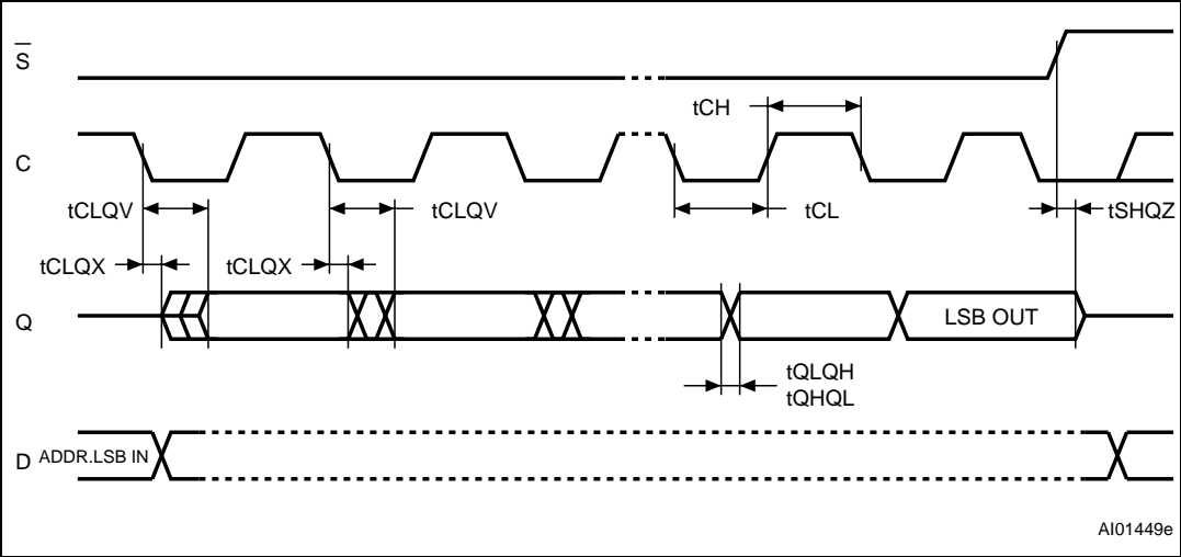
Figure 26. Output timing
