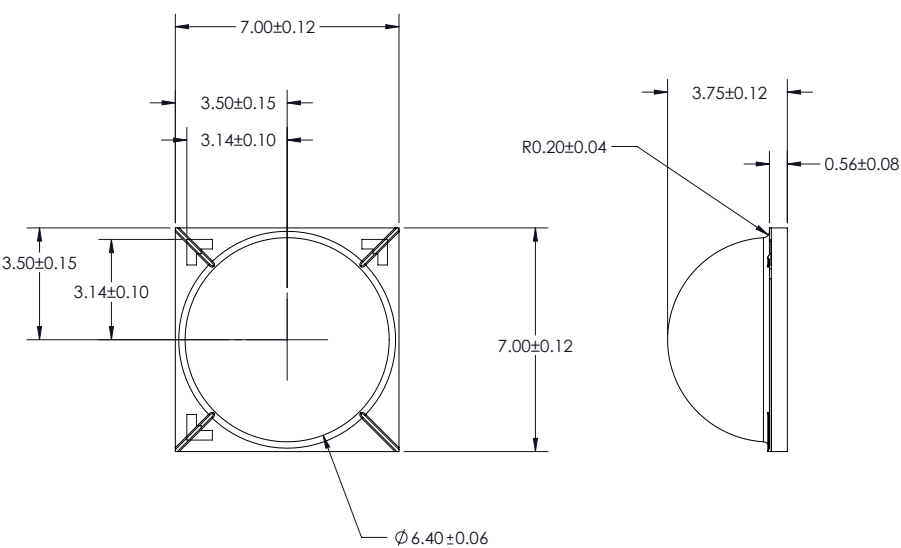
Figure 9. Mechanical dimensions for LUXEON M.
