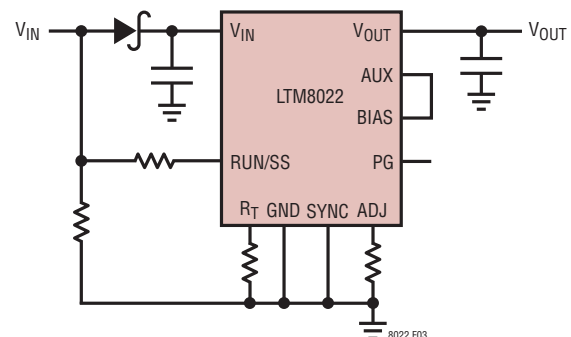
Figure 3. The Input Diode Prevents a Shorted Input from Discharging a Back-Up Battery Tied to the Output. It Also Protects the Circuit From a Reversed Input. The LTM8022 Runs Only When the Input is Present
