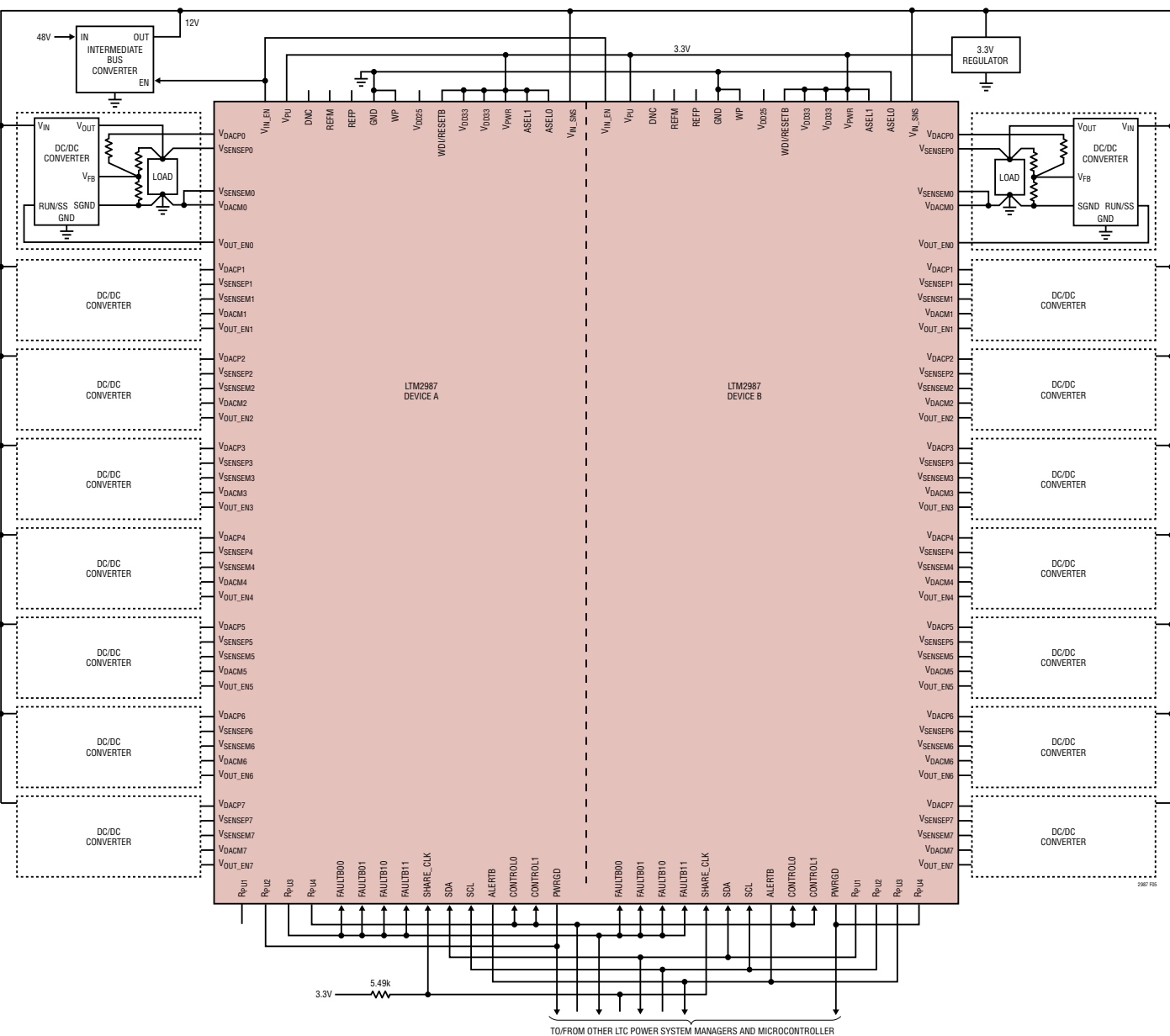
Figure 5. LTM2987 16-Channel Application Circuit with External 3.3V Chip Power
