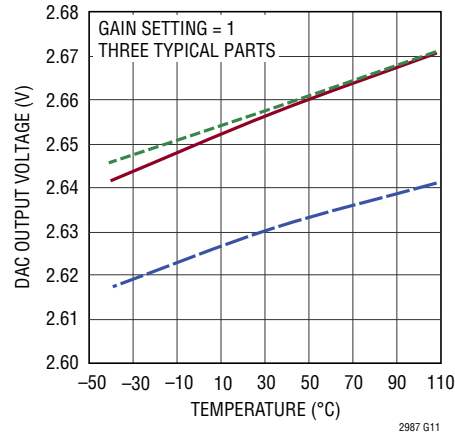
DAC Full-Scale Output Voltage vs Temperature
