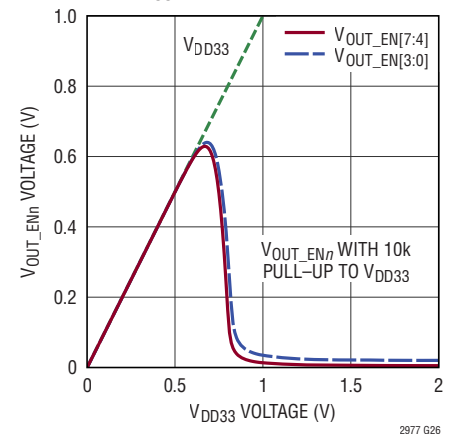
V OUT_EN[7:0] Output Voltage vs V DD33
