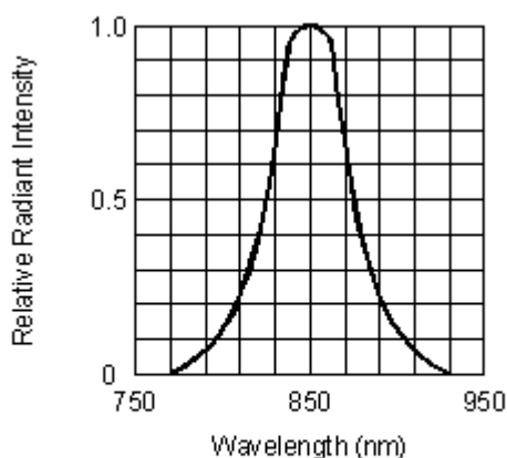
FIG.1 SPECTRAL DISTRIBUTION
