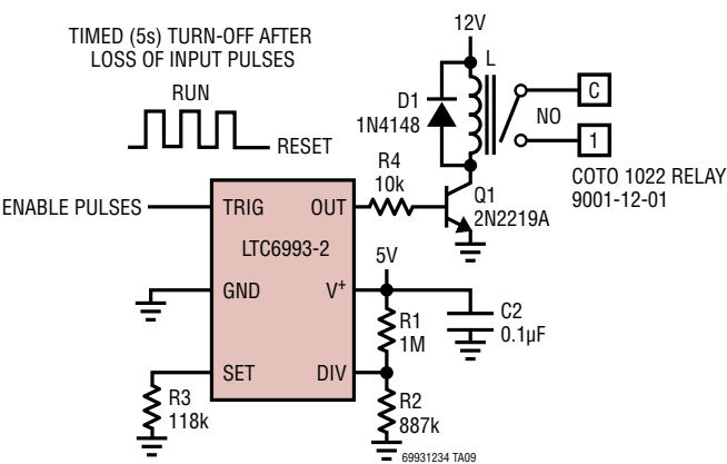
Safety Time-Out Relay Driver
