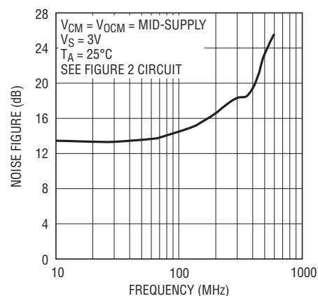
LTC6404-1 Noise Figure vs Frequency
