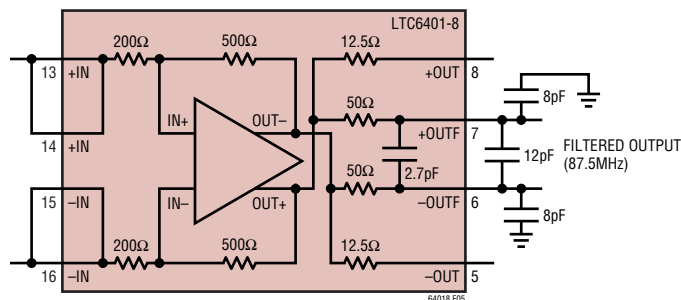
Figure 5. LTC6401-8 Internal Filter Topology Modified for Low Filter Bandwidth (Three External Capacitors)
