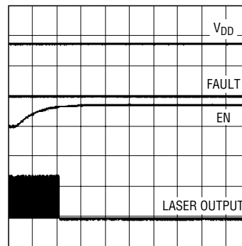
Transmitter Disable
