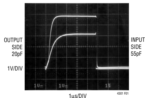
Figure 1. Input-Output Connection
