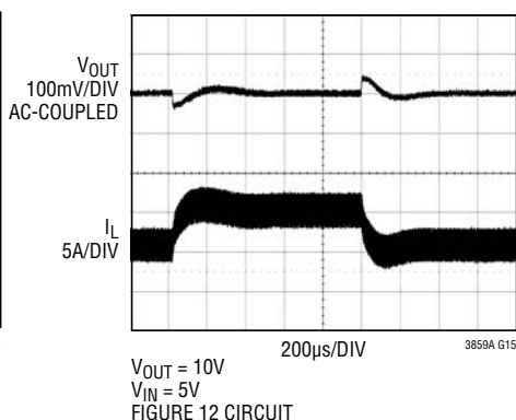
Load Step (Boost) Forced Continuous Mode
