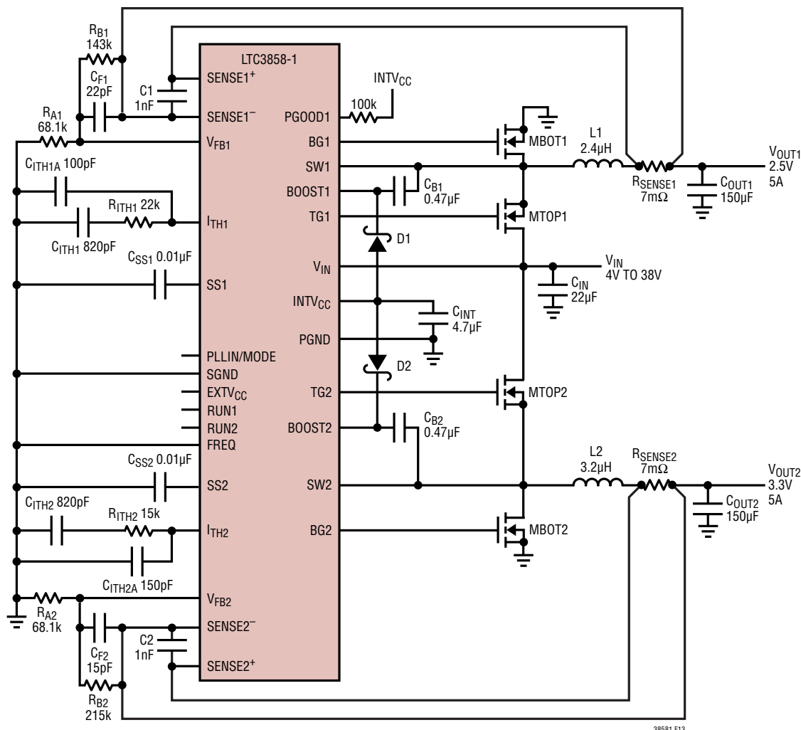
High Efficiency Dual 2.5V/3.3V Step-Down Converter
