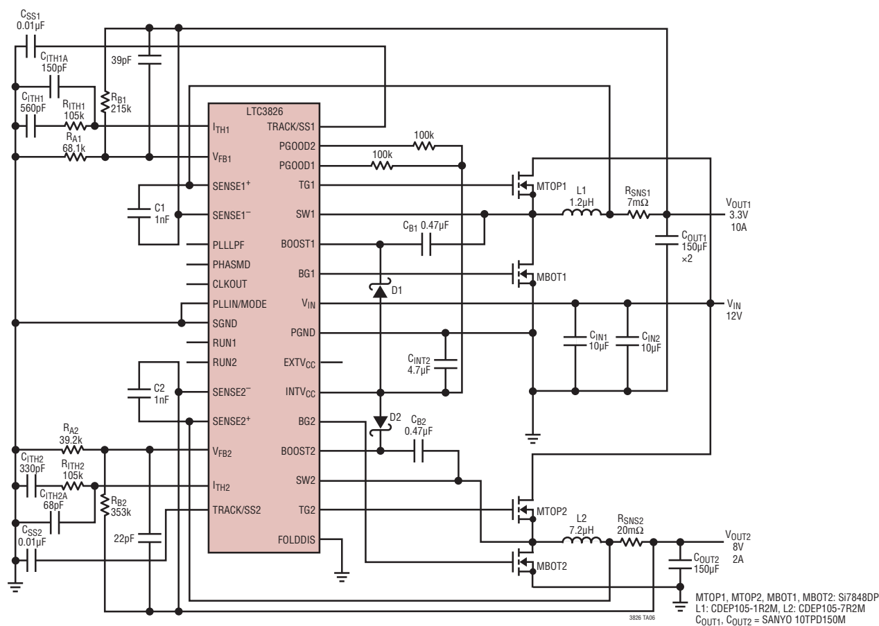
High Efficiency Dual 3.3V/8V Step-Down Converter
