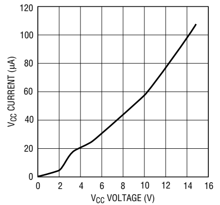
VCC Shutdown Current vs VCC Voltage
