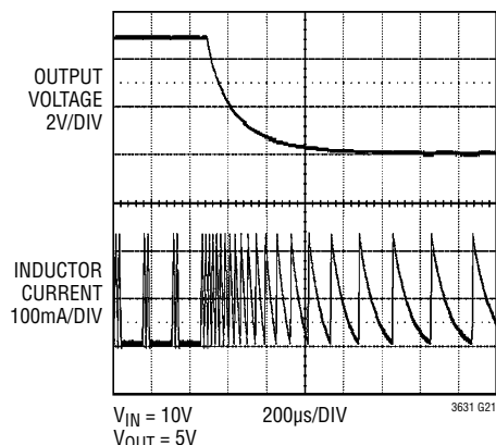
Short-Circuit Response
