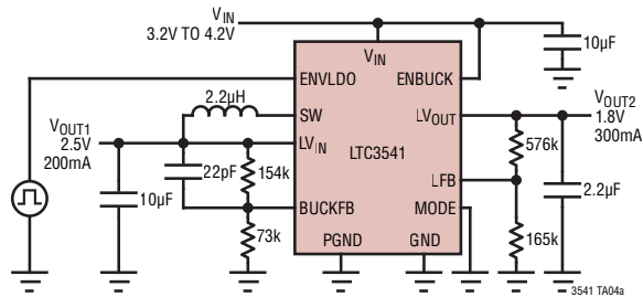
Dual Output Using Minimal External Components with V_{OUT2} Controlled by External Logic Signal, Buck in Burst Mode Operation for High Efficiency Down to Low Load Currents
