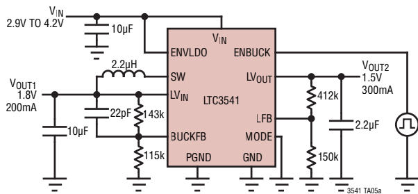
Dual Output Using Minimal External Components with V_{OUT1} Controlled by External Logic Signal, Buck in Burst Mode Operation for High Efficiency Down to Low Load Currents
