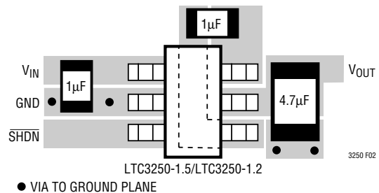
Figure 2. Recommended Layout
