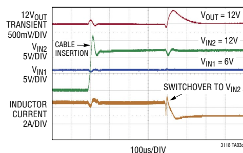
12V IN2 Inductive Cable Insertion with V OUT = 12V and 800mA Load
