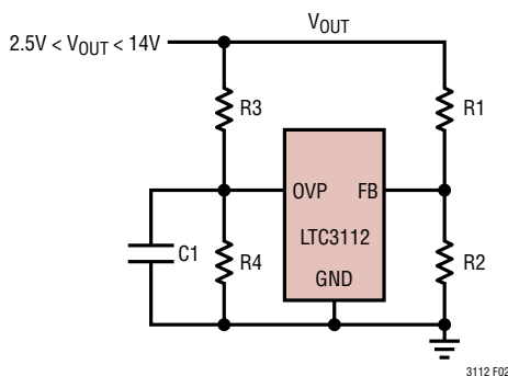
Figure 2. Setting the Output Voltage
