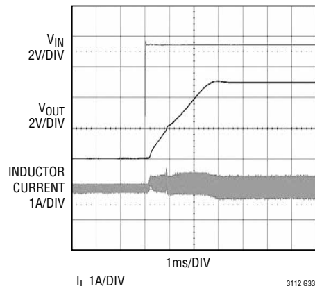
7.5V IN to 5.0V OUT Soft-Start Waveforms
