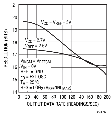
Figure 33. Resolution ( \text{INL}_{\text{MAX}} \leq 1\text{LSB} ) vs Output Data Rate and Reference Voltage
