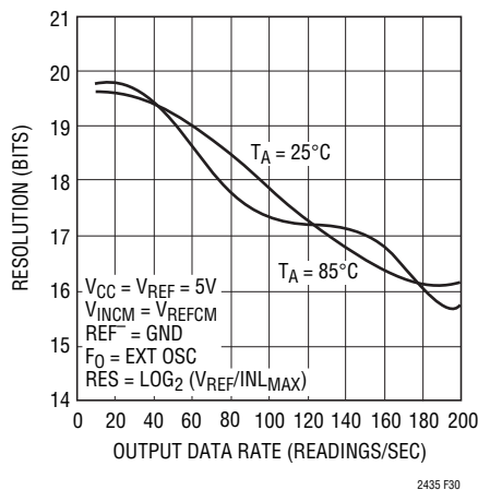
Figure 30. Resolution ( \text{INL}_{\text{RMS}} \leq 1\text{LSB} ) vs Output Data Rate and Temperature
