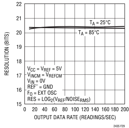
Figure 29. Resolution ( \text{Noise}_{\text{RMS}} \leq 1\text{LSB} ) vs Output Data Rate and Temperature
