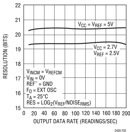
Figure 32. Resolution ( \text{Noise}_{\text{RMS}} \leq 1\text{LSB} ) vs Output Data Rate and Reference Voltage
