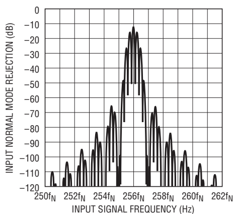
Figure 36. Input Normal Mode Rejection
