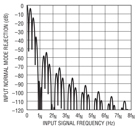
Figure 35. Input Normal Mode Rejection
